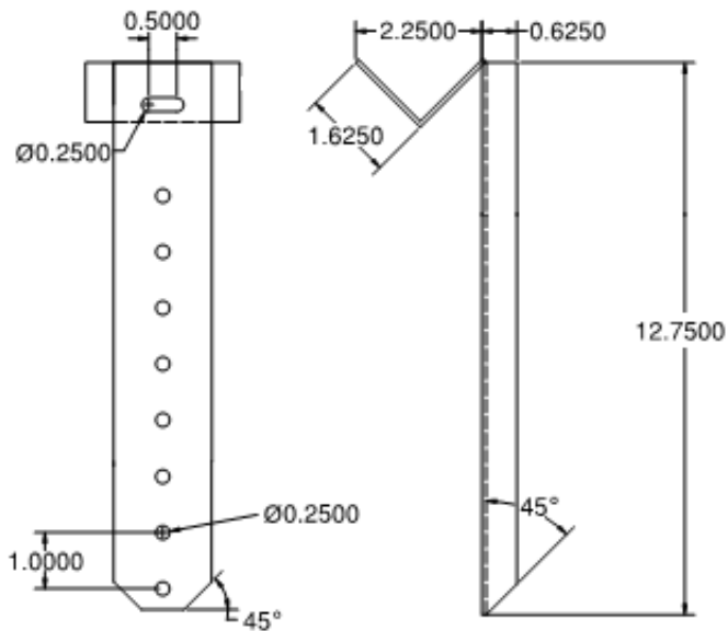
Mounting Bracket
